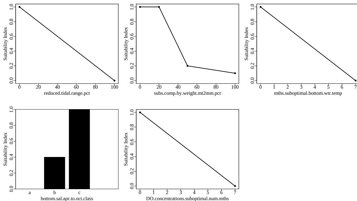
Figure 1. Suitability index graphs for variables included in the englishsoleJuvImpactAlt model in ecorest .
